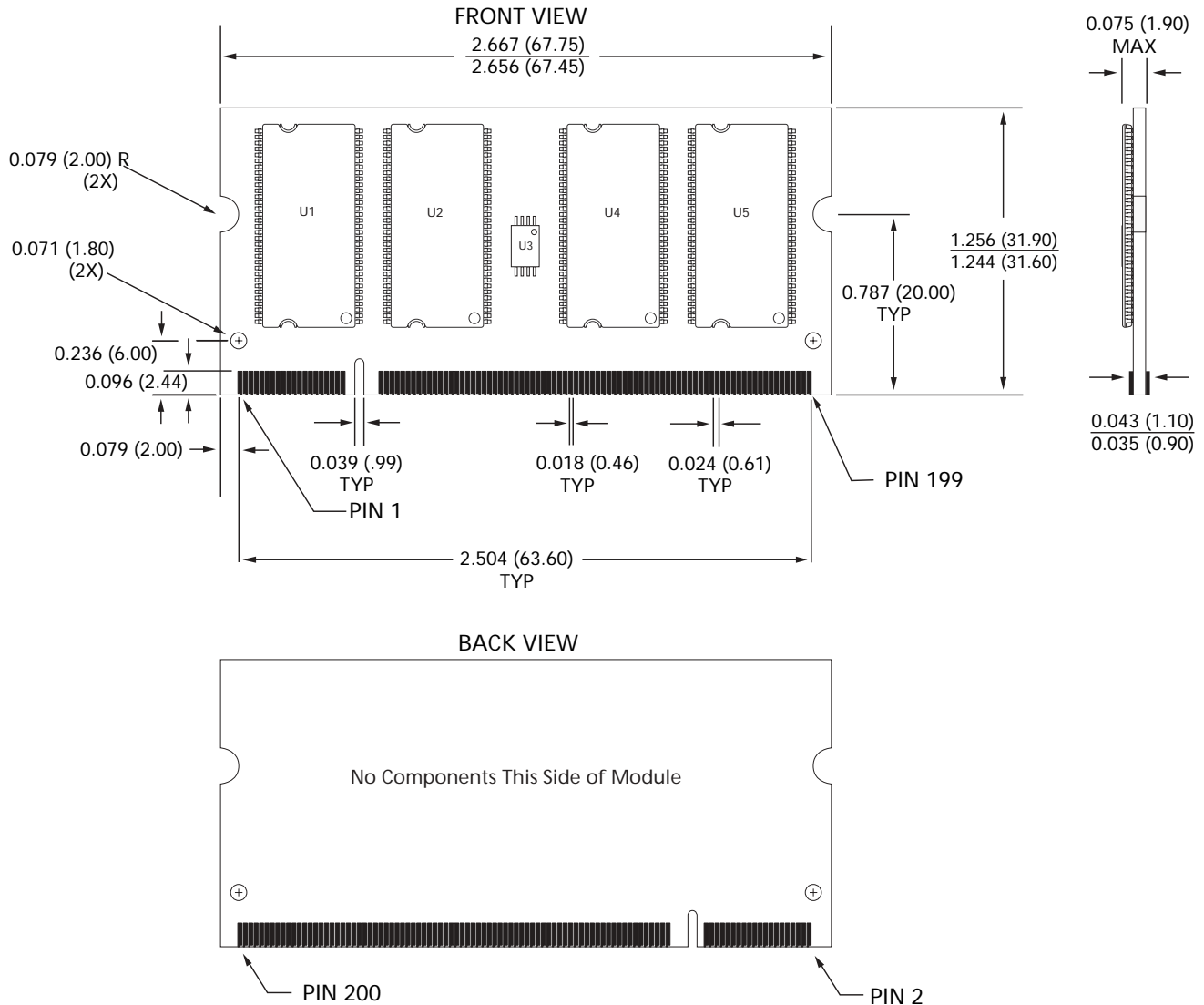
Figure 16: 200-Pin SODIMM Dimensions
