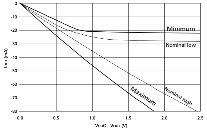
Figure 10: Reduced Output Pull-Up Characteristics
