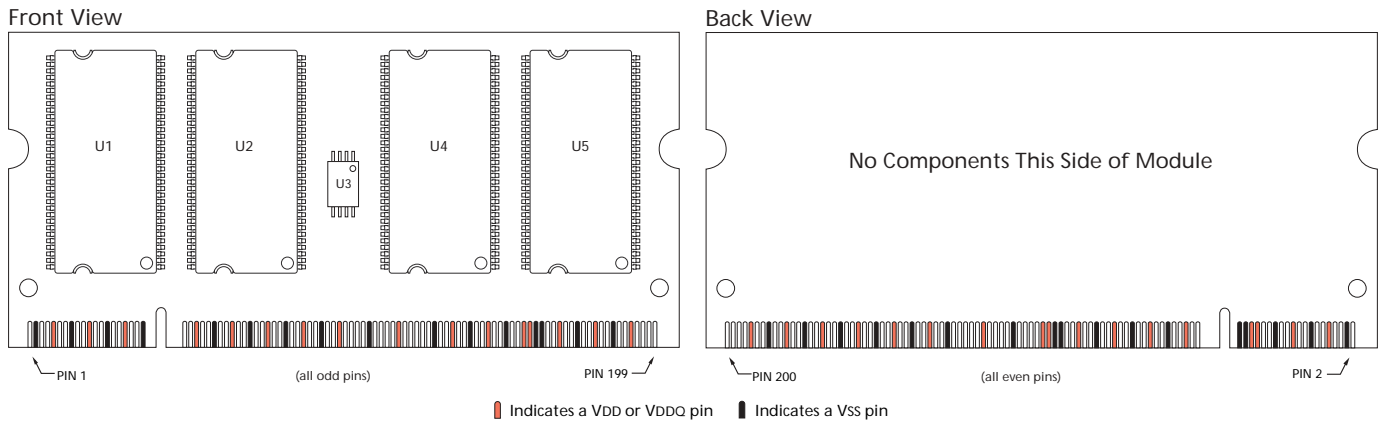
Figure 2: 200-Pin SODIMM Module Layout
